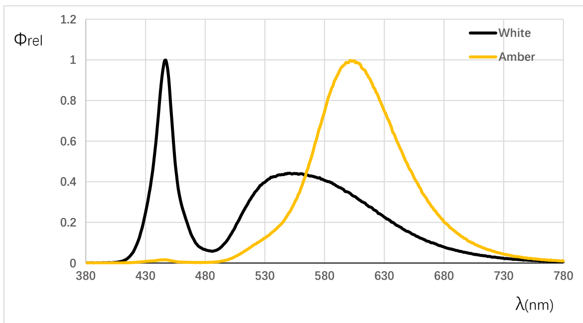
Fig 2. 相对发光光谱 Relative Spectral Distribution vs. Wavelength
