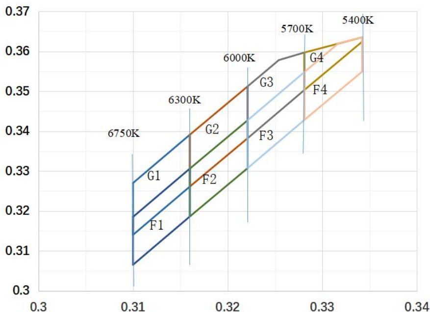
AGL Series Color Chromaticity Groups
