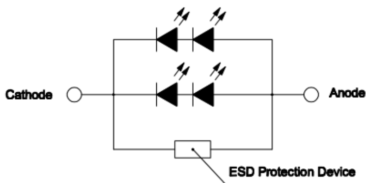
6V Circuit Configuration 6V Circuit Configuration
