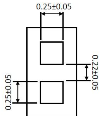
Meter solder stencil aperture
