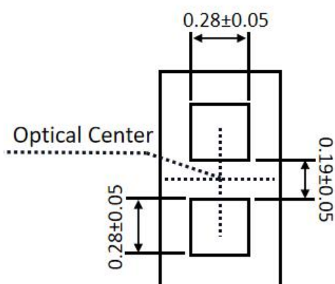
Soldering pad design
