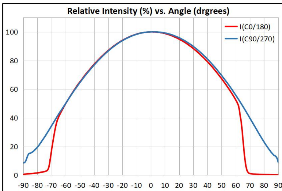
Fig 2. 辐射特性 Radiation Pattern Characteristics
