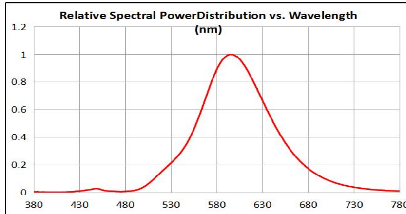
Fig 1. 相对发光光谱/ Relative Spectral Power Distribution vs. Wavelength
