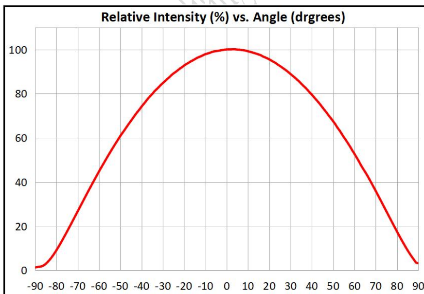
Fig 2. 辐射特性 Radiation Pattern Characteristics
